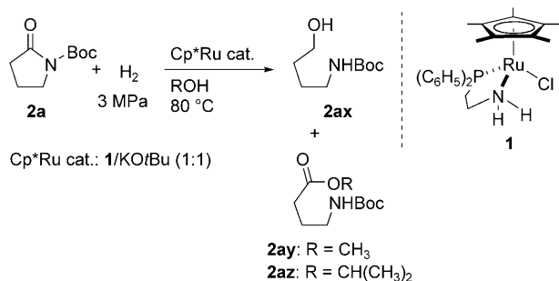
Scheme 2. Hydrogenation of 2a with [\text{Cp}^*\text{Ru(PN)}] in various alcoholic solvents.
